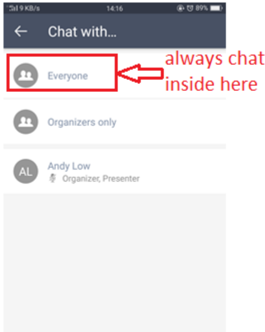
Figure 7: Chat System
